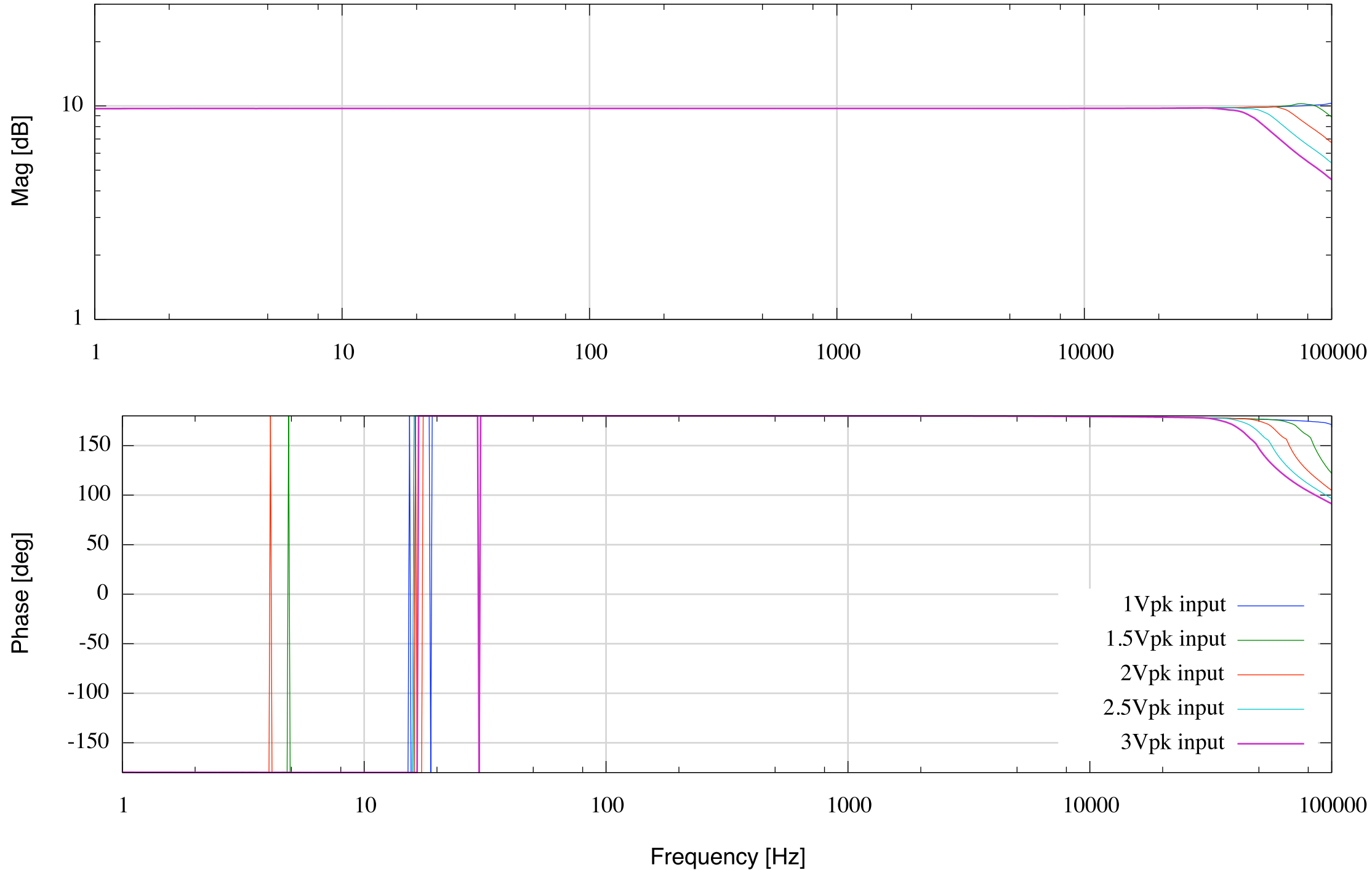
TF of High voltage amplifier used for laser PZT input
