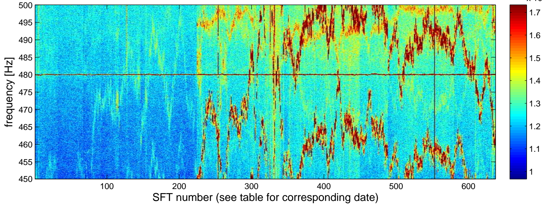
Spectrogram for H1:hof; GPS 851803214 – 853358414 s.
