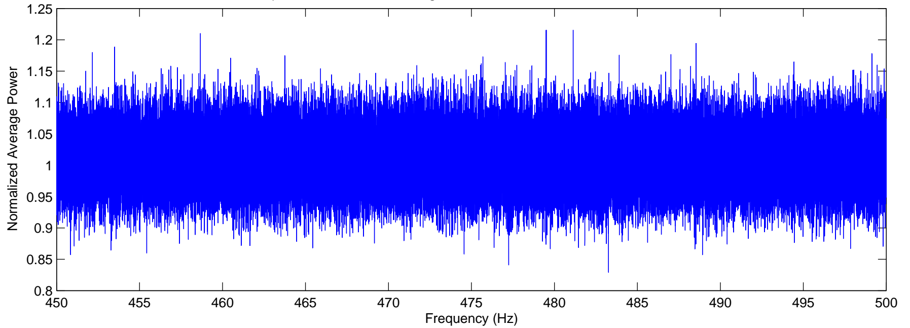
Spectrum for H1:hof; averaged over GPS 851803214 – 853358414 s.
