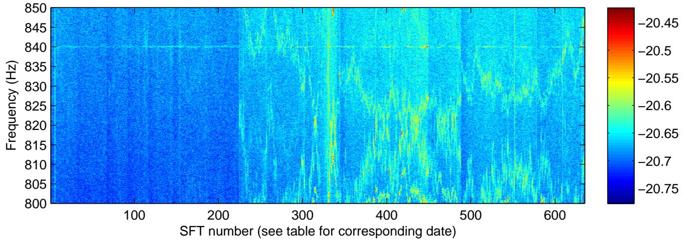
Spectrum for H1:hoft; averaged over GPS 851803214 – 853358414 s.
