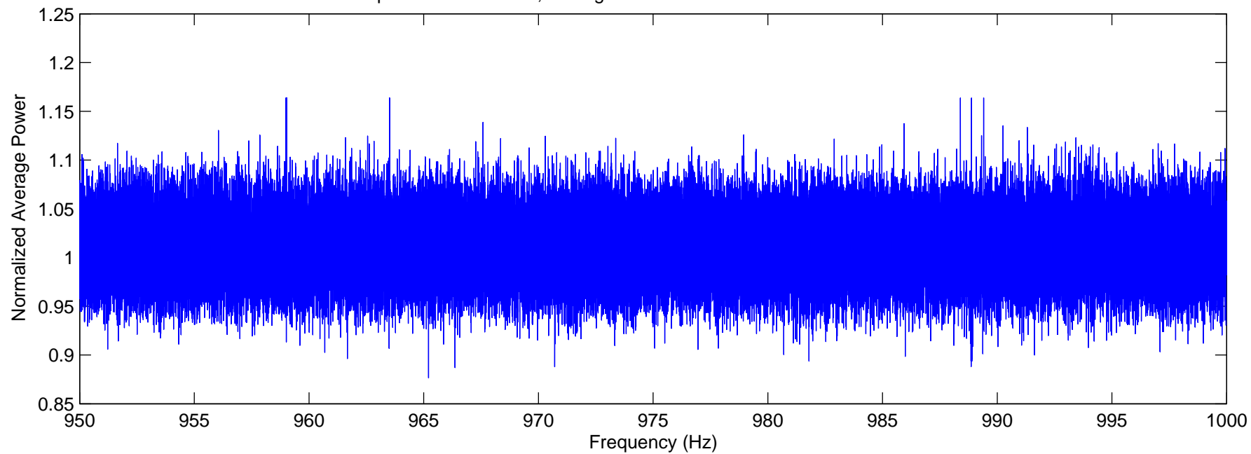
Spectrum for H1:hoft; averaged over GPS 841104014 – 843696014 s.
