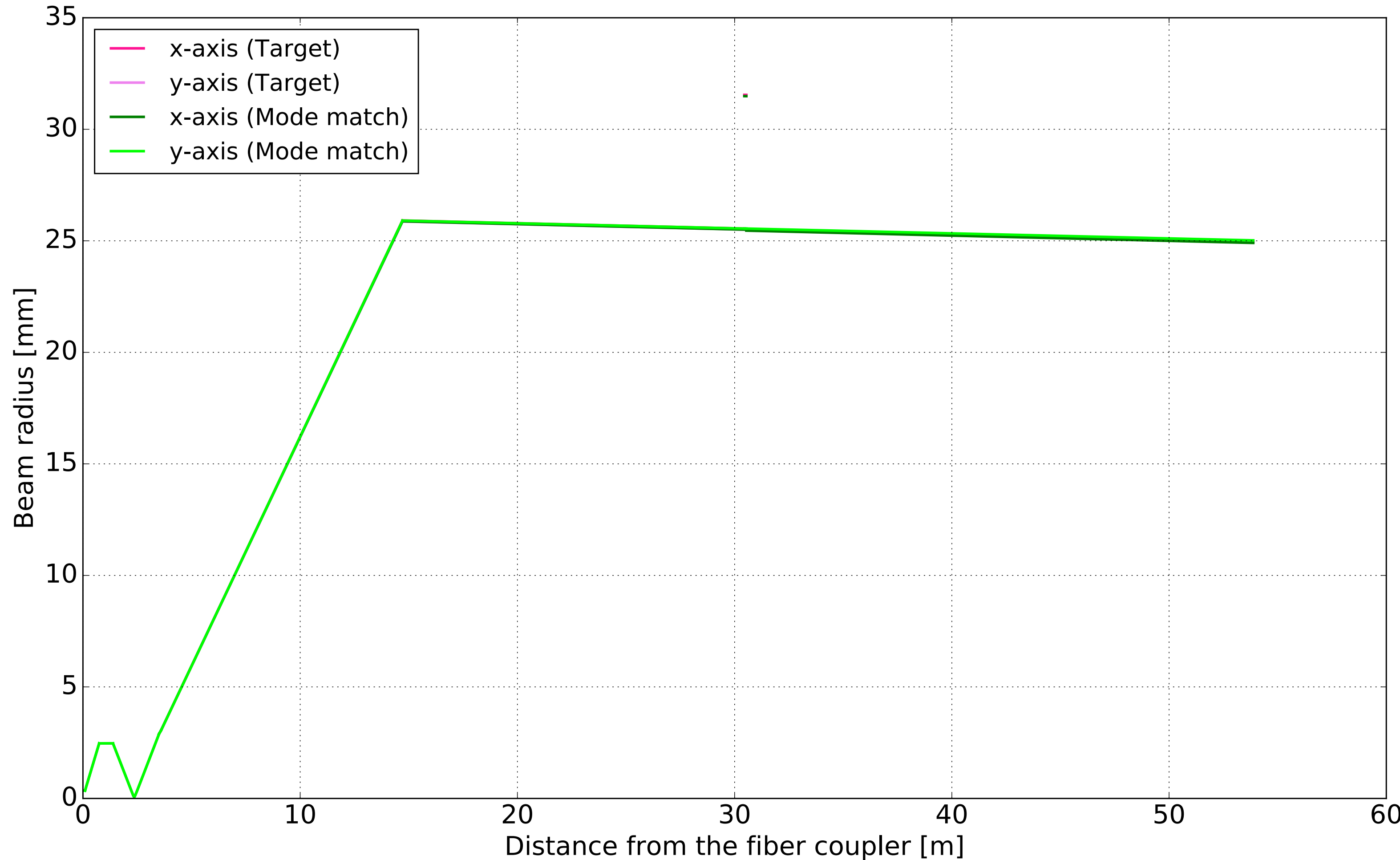
From the fiber coupler to ITMY
